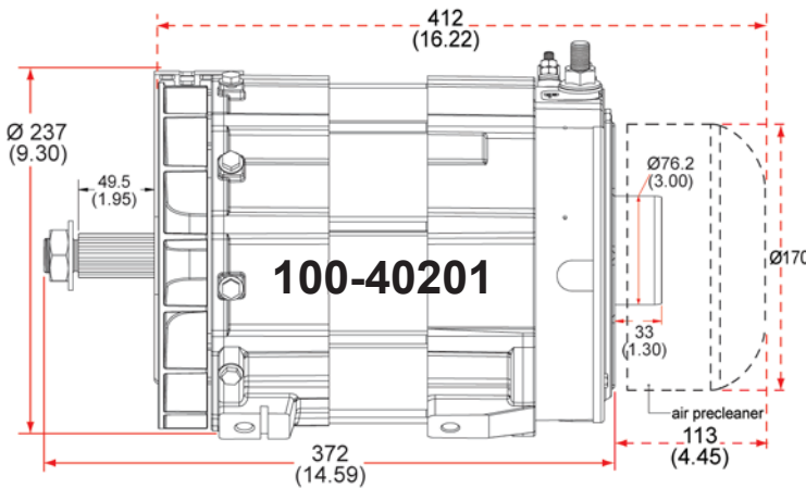
Dimensions are listed in mm over (in)
